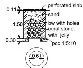
percolation pit
