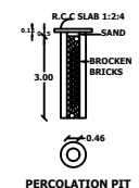
PERCOLATION PIT
