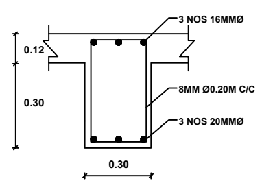
ROOF BEAM DETAILS
