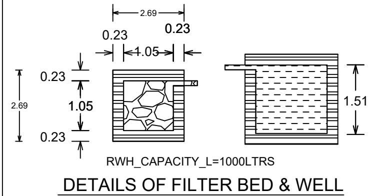
DETAILS OF FILTER BED & WELL
