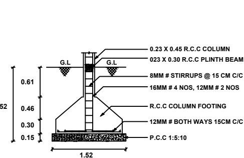
COLUMN FOOTING DETAILS
