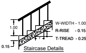
Staircase Details
