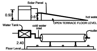
Details of solar water heating system
