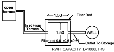
Plan Of Filter Bed & Well
