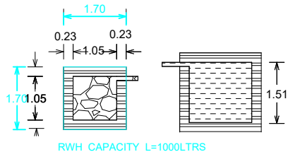
DETAILS OF FILTER BED & WELL
