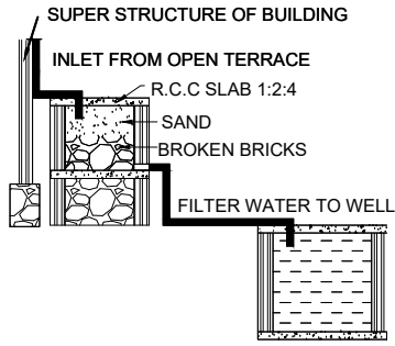
RAINWATER HARVESTING
