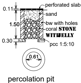
percolation pit
