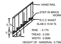
STAIR DETAILS
