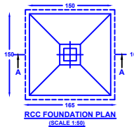
RCC FOUNDATION PLAN
