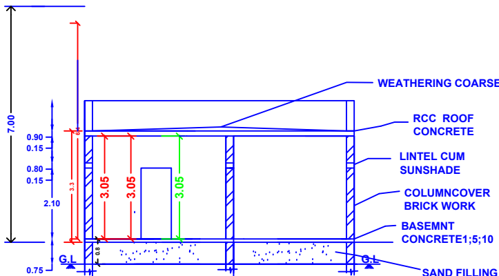
SECTION AB
