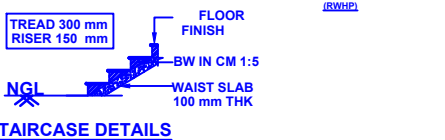
STAIRCASE DETAILS
