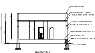
SECTION S-S
