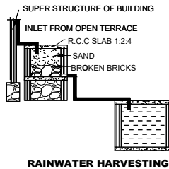
RAINWATER HARVESTING
