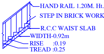
STAIR DETAIL
