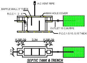
SEPTIC TANK & TRENCH
