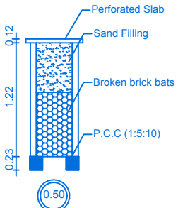
RAIN WATER COLLECTION WELL
