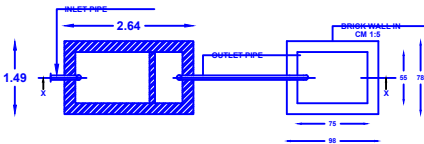
SECTION-YY SEPTIC TANK AND D-TRENCH DETAILS (SCALE 1 : 100)
