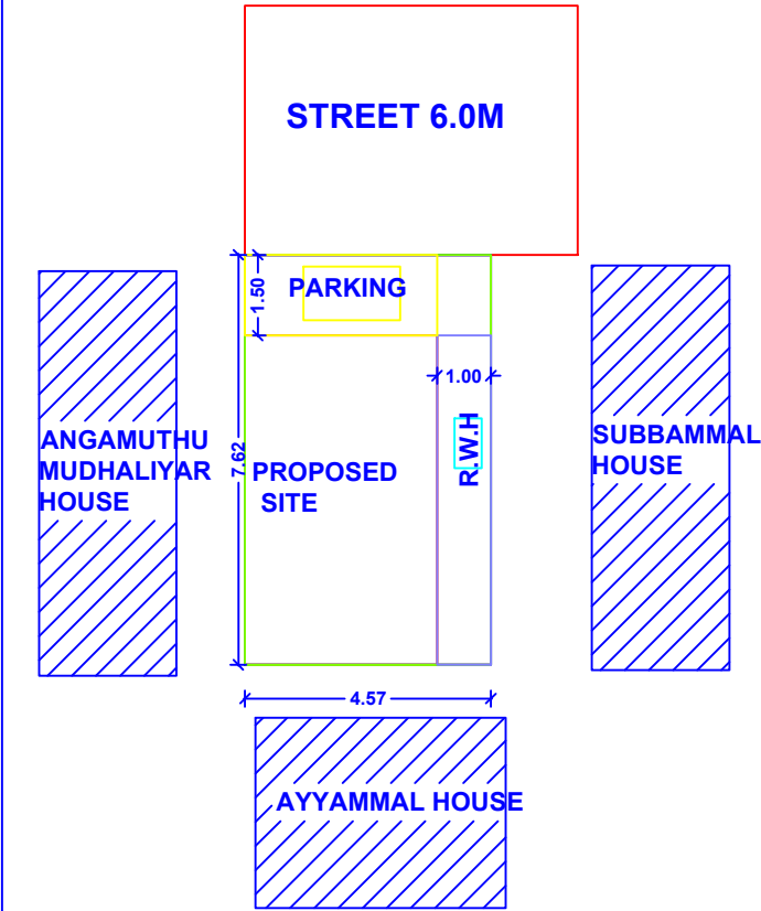
SITE PLAN
