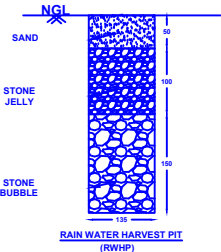
RAIN WATER HARVEST PIT (RWHP)
