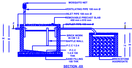
SECTION-XX
