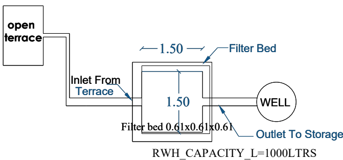
Plan Of Filter Bed & Well
