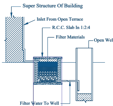
Details Of Rainwater Harvesting System
