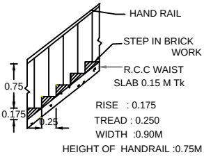
STAIR DETAILS
