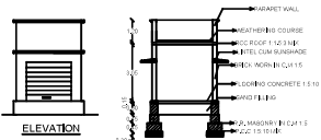
SECTION ON AB
