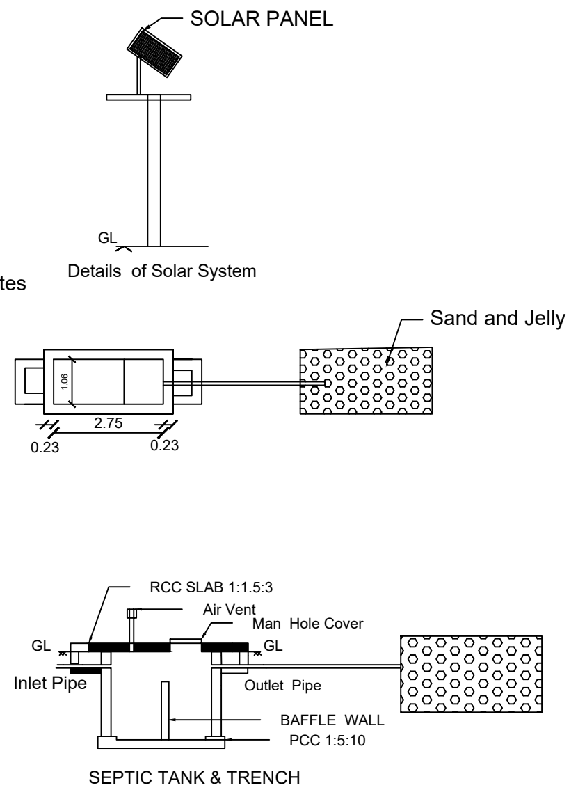
SEPTIC TANK & TRENCH
