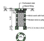
PERCOLATION PIT FOR 30 Sq. m. (Scale:- 1:50)
