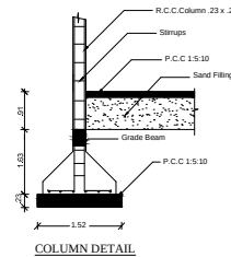
COLUMN DETAIL
