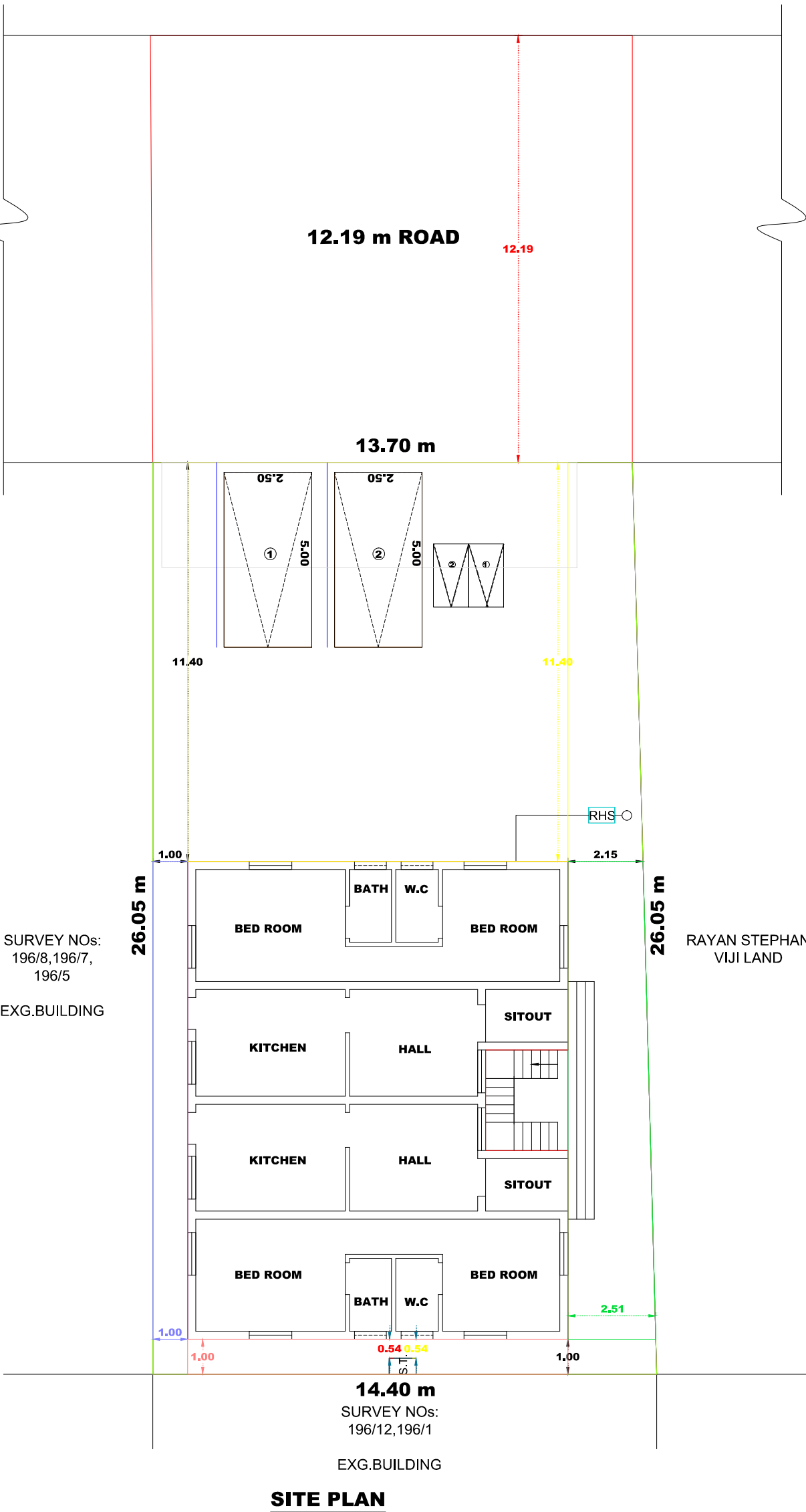
SITE PLAN
