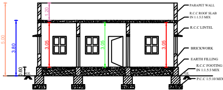
SECTION ON AA
