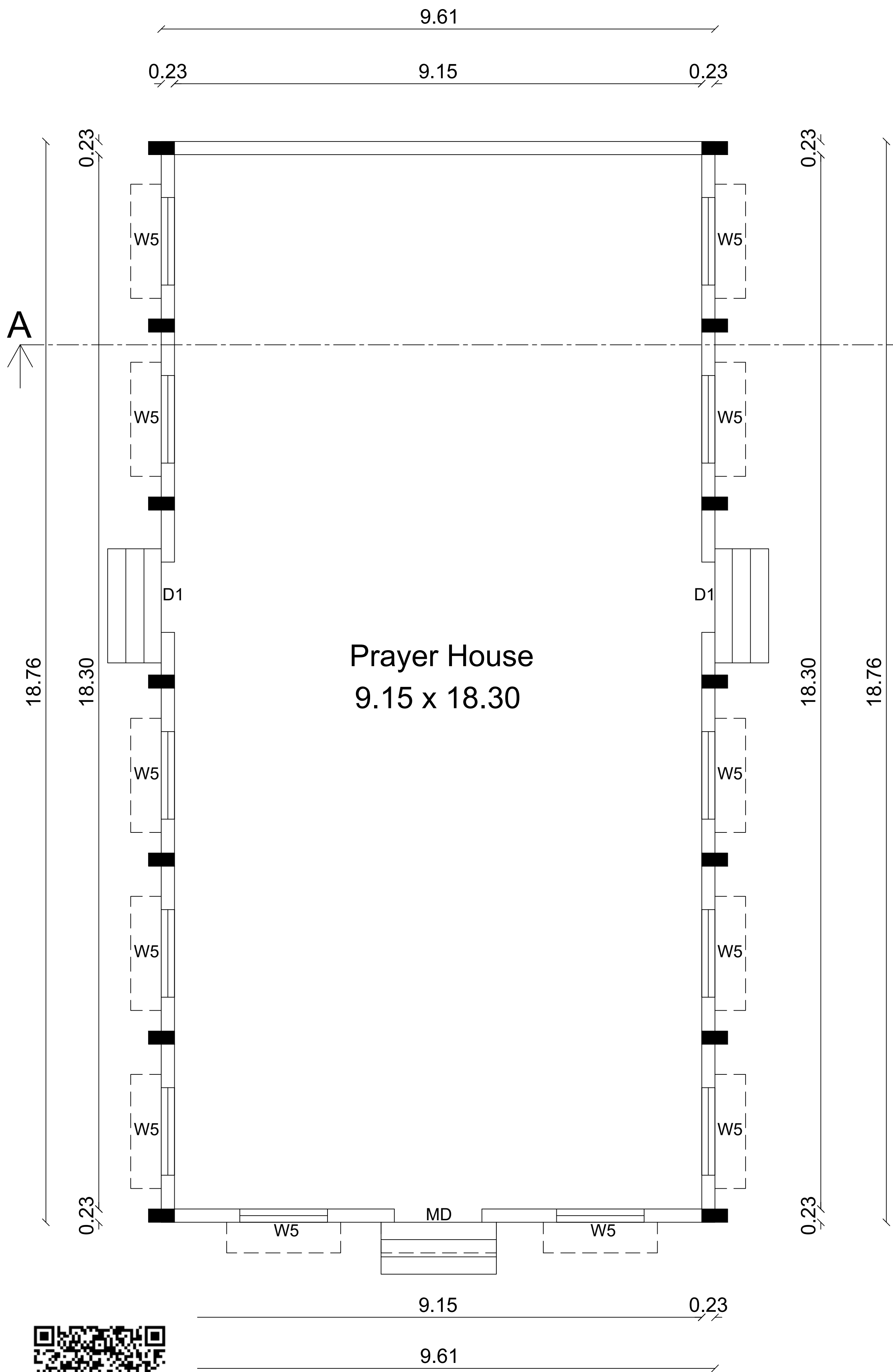
PLAN
