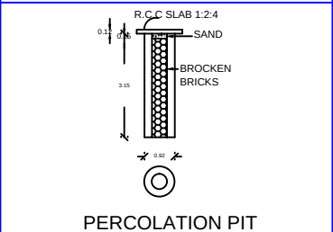
PERCOLATION PIT
