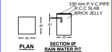
SECTION OF RAIN WATER PIT
