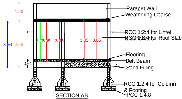
SECTION AB
