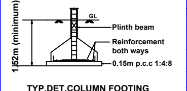
TYP.DET.COLUMN FOOTING
