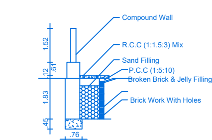
RAIN WATER HARVEST DETAILS
