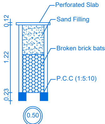
RAIN WATER COLLECTION WELL
