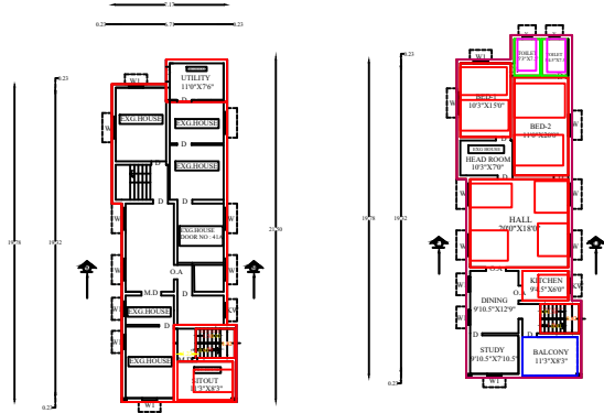
EXG & PRO.GROUND FLOOR PLAN
