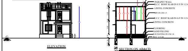
SECTION ON AB&CD
