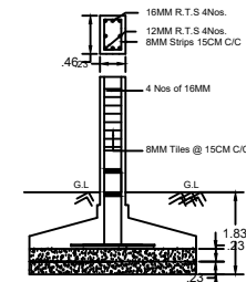
RCC COLUMN DETAILS
