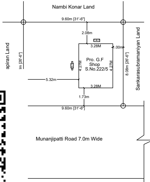
SITE PLAN
