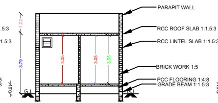
SECTION BLOCK-2
