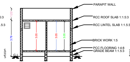
SECTION BLOCK-3
