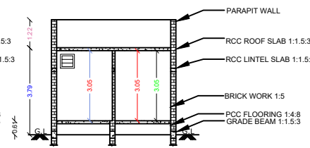
SECTION BLOCK-4
