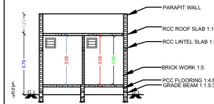
SECTION BLOCK-1
