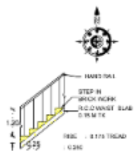
STAIR DETAILS
