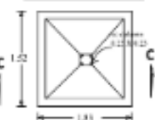
Details of column footing
