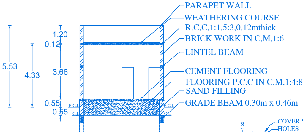
SECTION ON"AA"
