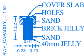
SECTION OF RAIN WATER COLLECTION TANK
