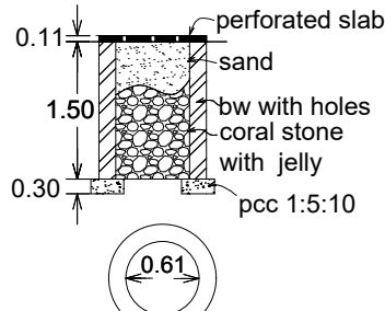
percolation pit
