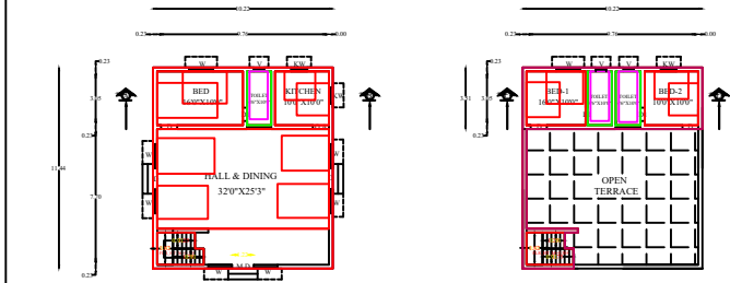
PRO.GROUND FLOOR PLAN
