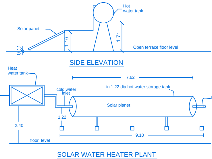
SOLAR WATER HEATER PLANT
