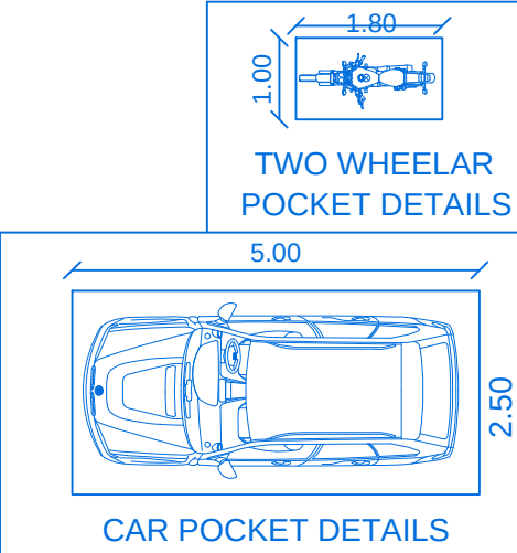
CAR POCKET DETAILS ALL DIMENSIONS ARE IN METRE SCALE 1:100
