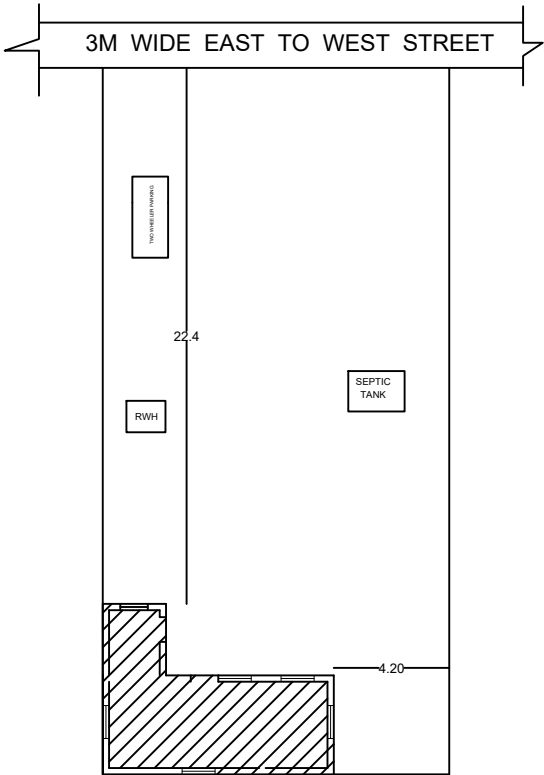
SITE PLAN
