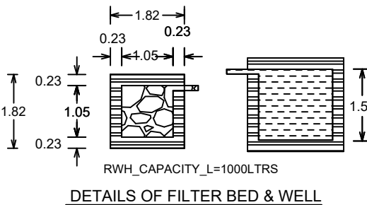
DETAILS OF FILTER BED & WELL
