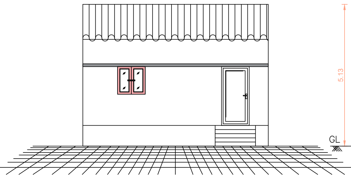
FRONT ELEVATION.
