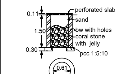
PERCOLATION PIT
