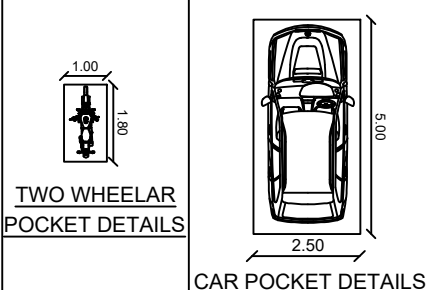
CAR POCKET DETAILS
