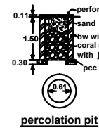
percolation pit
