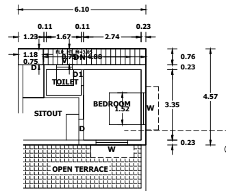
1 ST FLOOR PLAN
