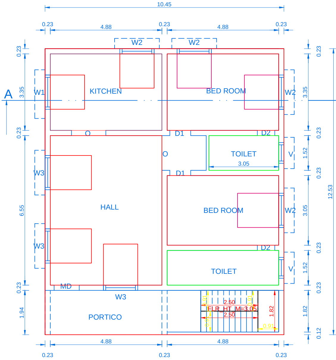
FLOOR PLAN
