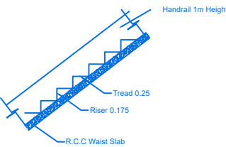
STAIR DETAILS
