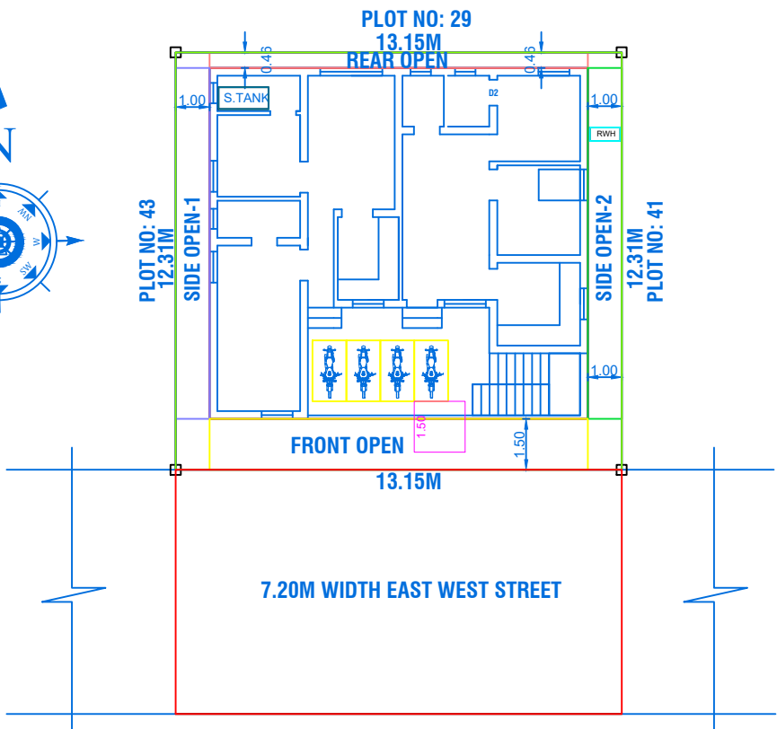
SITE PLAN(1:100)
