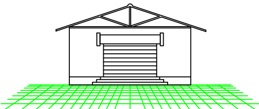
FRONT ELEVATION
