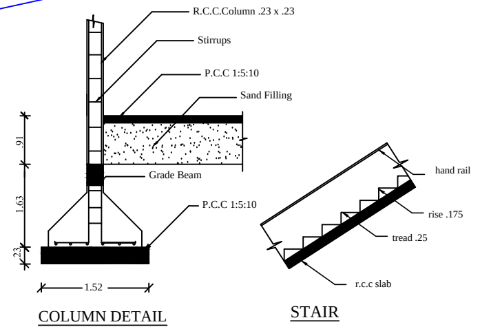
COLUMN DETAIL
