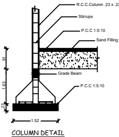
COLUMN DETAIL
