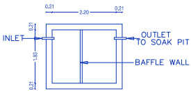
PLAN SEPTIC. TANK
