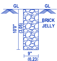
PERCUSSION PIT
