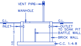
SECTION OF SEP.TANK
