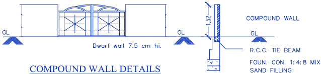
SECTION
