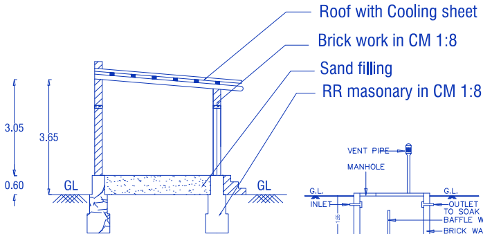
CROSS SECTION ON 'AB'
