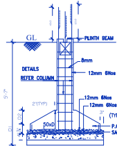
FOUNDATION DETAILS SCALE : 1:50.
