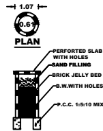
SECTION OF RAIN WATER COLLECTION TANK
