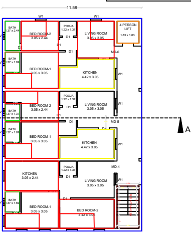
PROPOSED SECOND FLOOR
