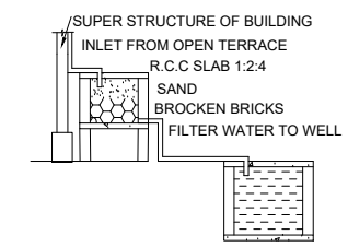
DETAILS OF FILTER BED & WELL
