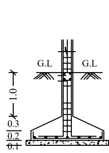
COLUMN FOOTING DETAILS - N.T.S
