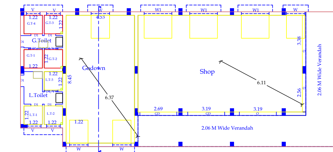
Prop.Ground Floor
