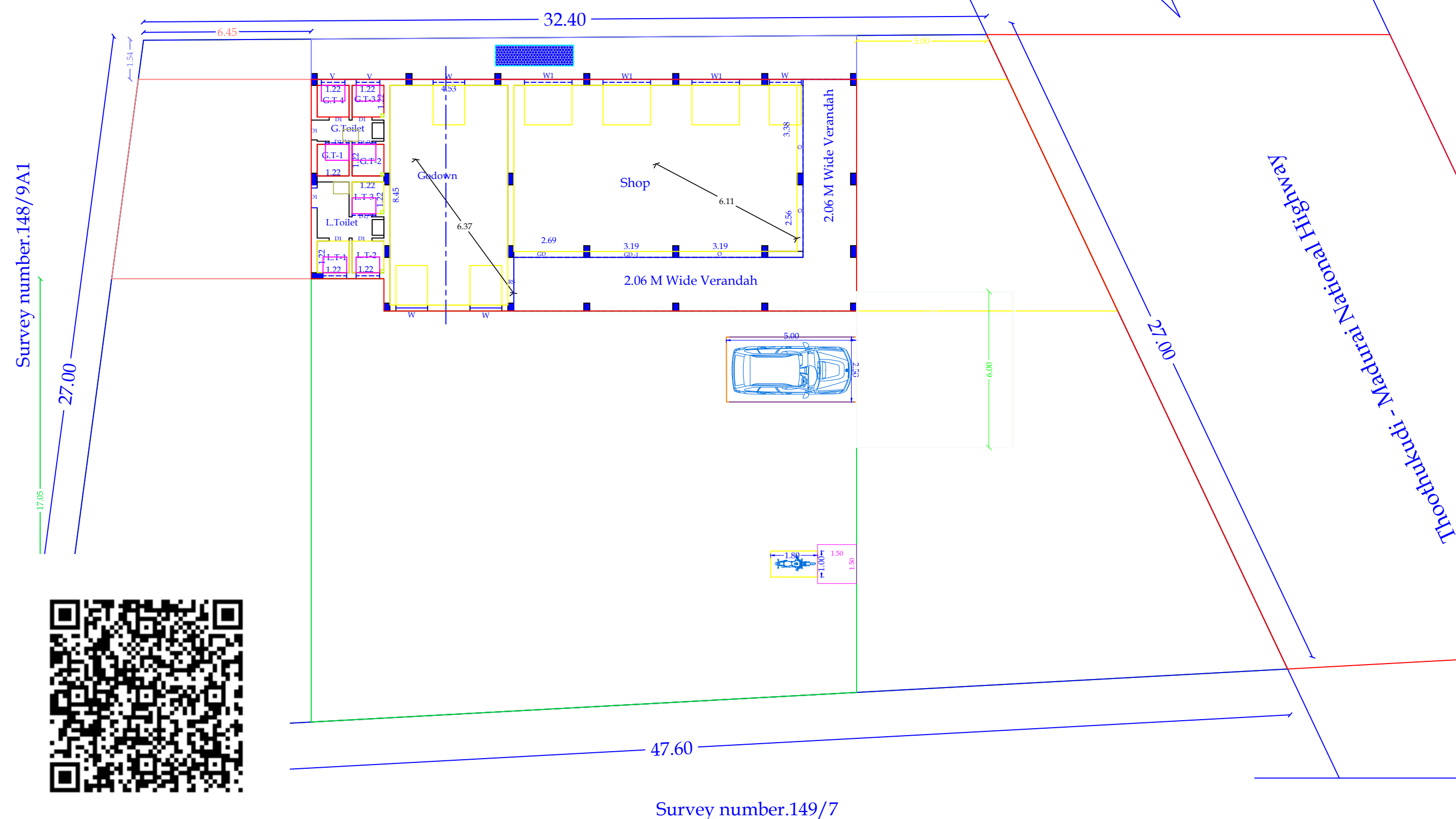
Prop.Ground Floor
