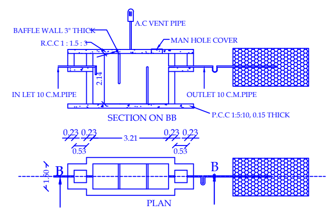
EXIS. SEPTIC TANK AND TRENCH & U TRAP ADOPTED
