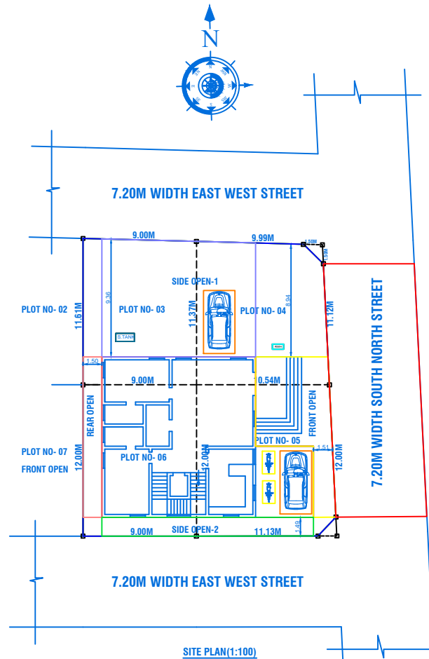
SITE PLAN(1:100)
