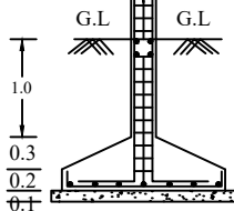
COLUMN FOOTING DETAILS - N.T.S
