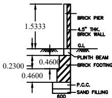
COMPOUND WALL DETAILS - N.T.S
