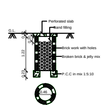
PERCOLATION PIT FOR 30 Sq. m. (Scale:- 1:50)
