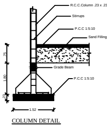
COLUMN DETAIL
