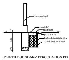
PLINTH BOUNDARY PERCOLATION PIT
