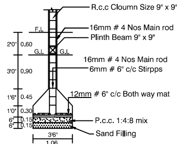
COLUMN DETIAL NOT TO SCALE
